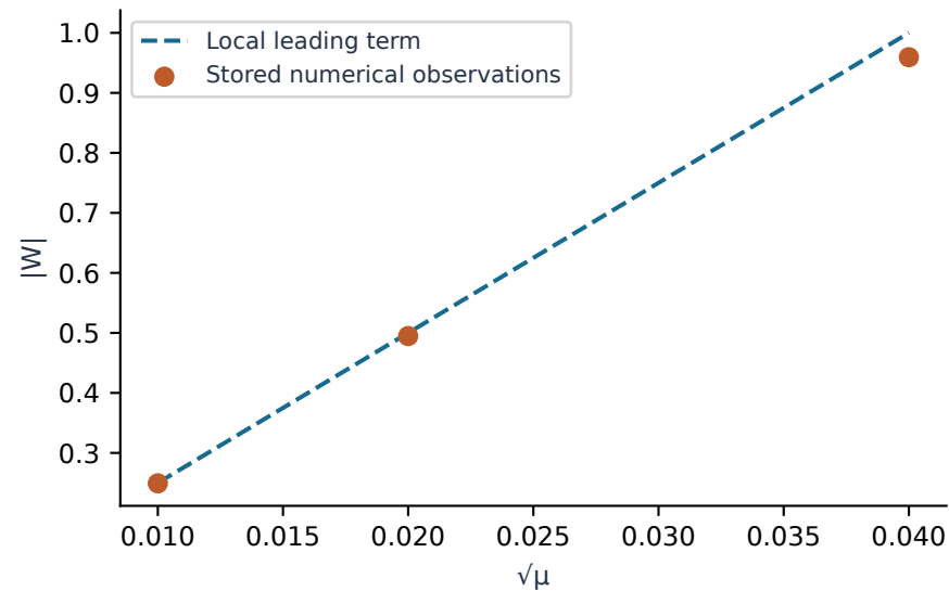
(a) M2 numerical onset versus asymptotic
