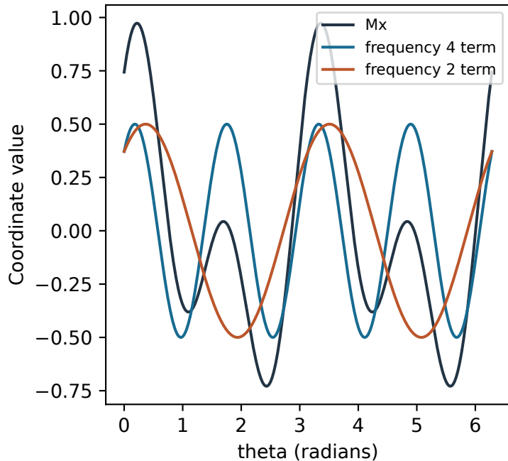
Exact product-to-sum decomposition
