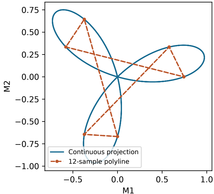
Three-petal rose, frozen amplitude
