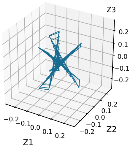
Z_macro
