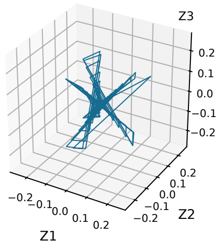
Z_total
