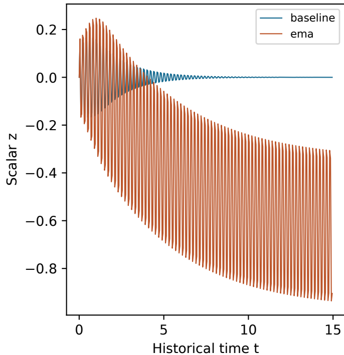
Same Omega; different historical Z
