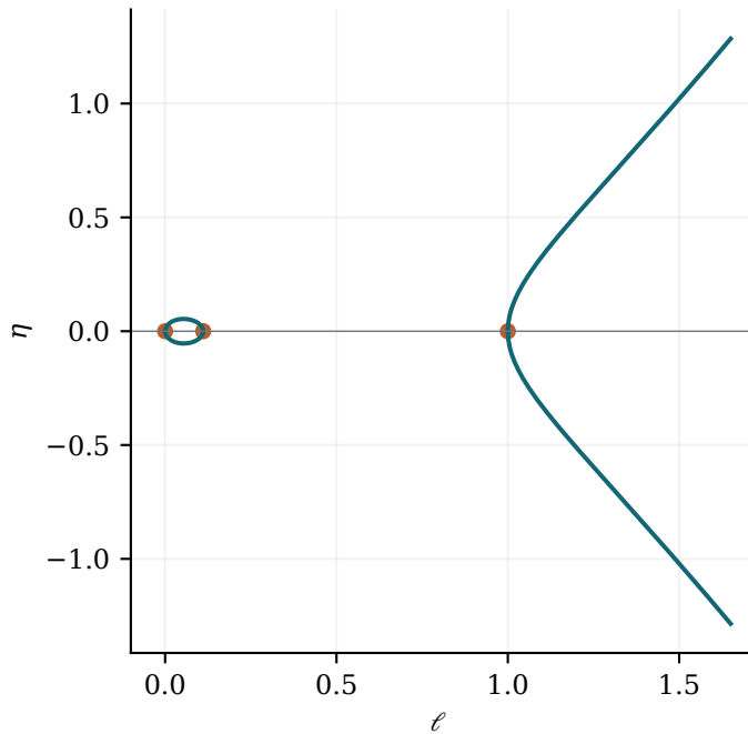
Legendre, m = 1/9
