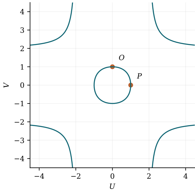
Edwards, t = 1/2
