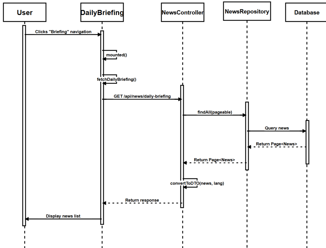
SD-01: View Daily Briefings
