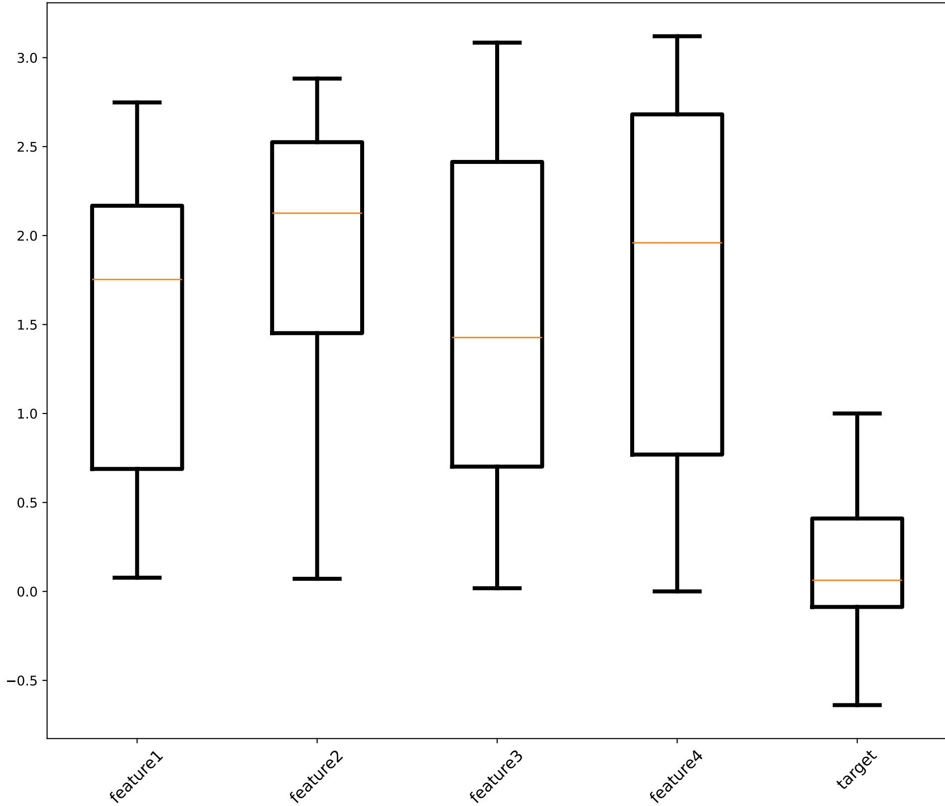
Validation Set
