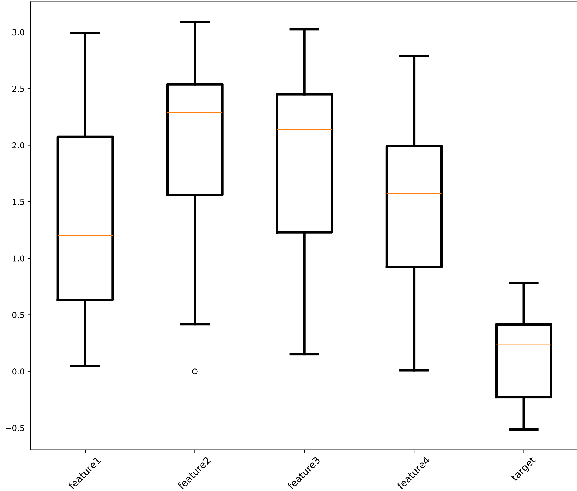
Test Set
