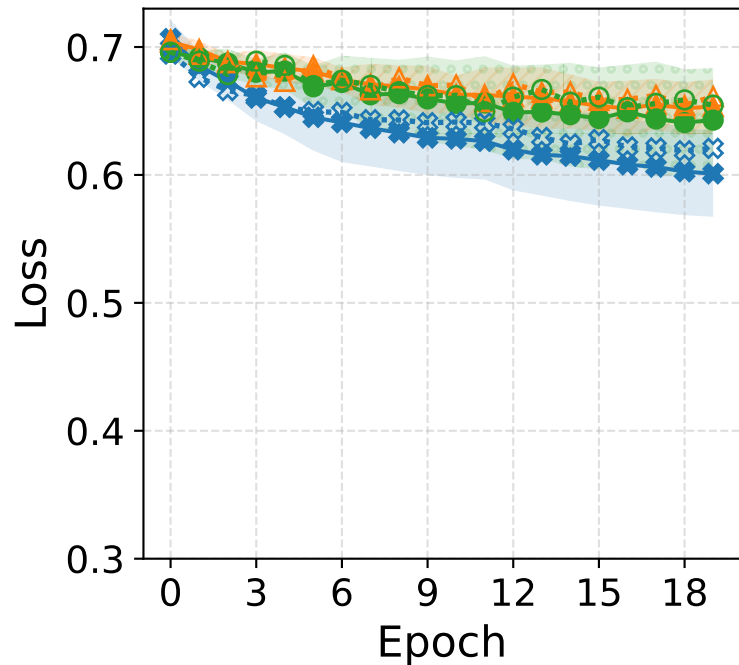
Model: QCNN
