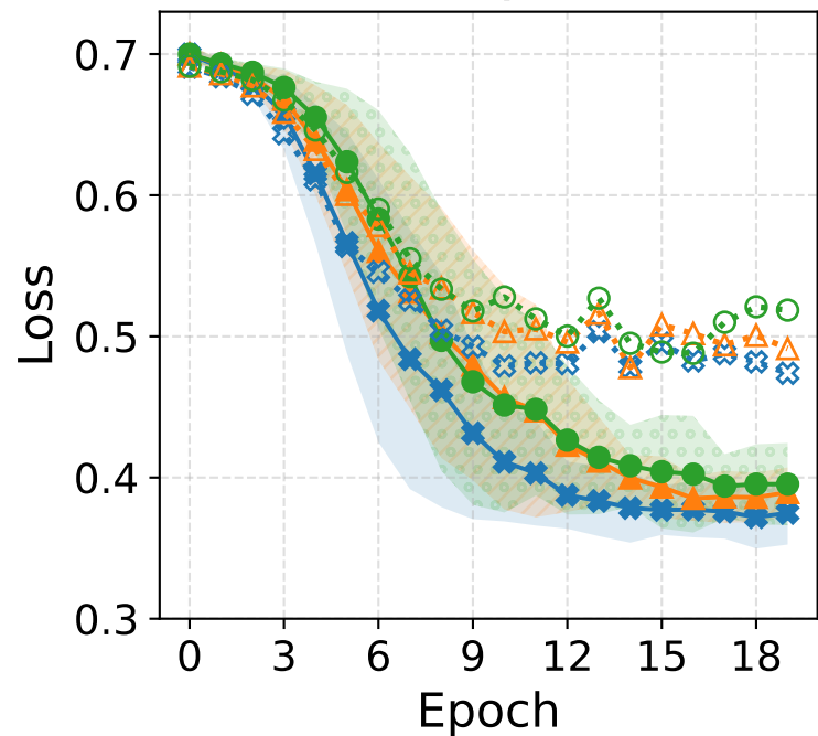
Model: HQCNN-EM
