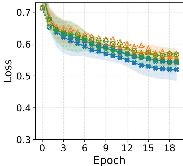
Model: QCNN
