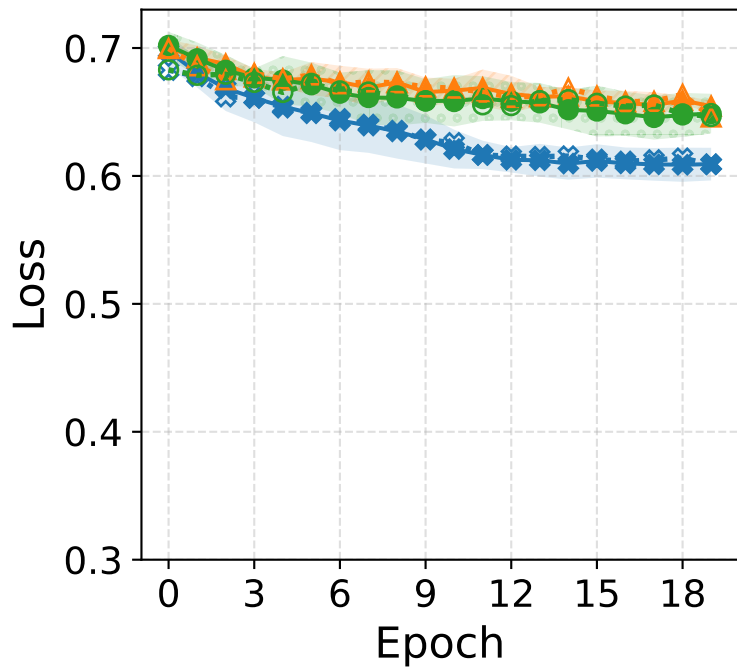
Model: QCNN
