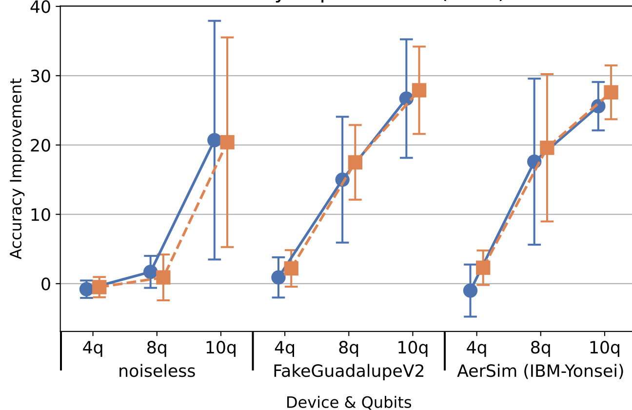
Accuracy Improvement (Train)
