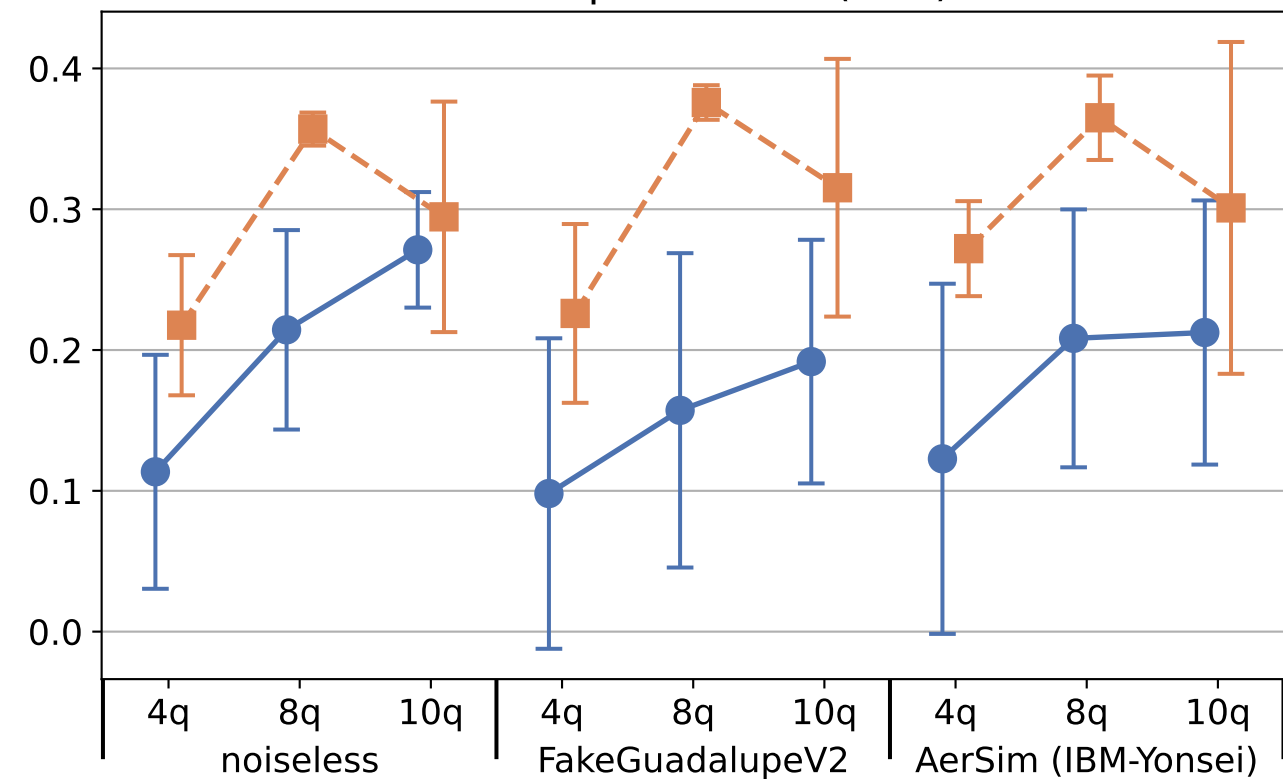
BCE Improvement (Test)
