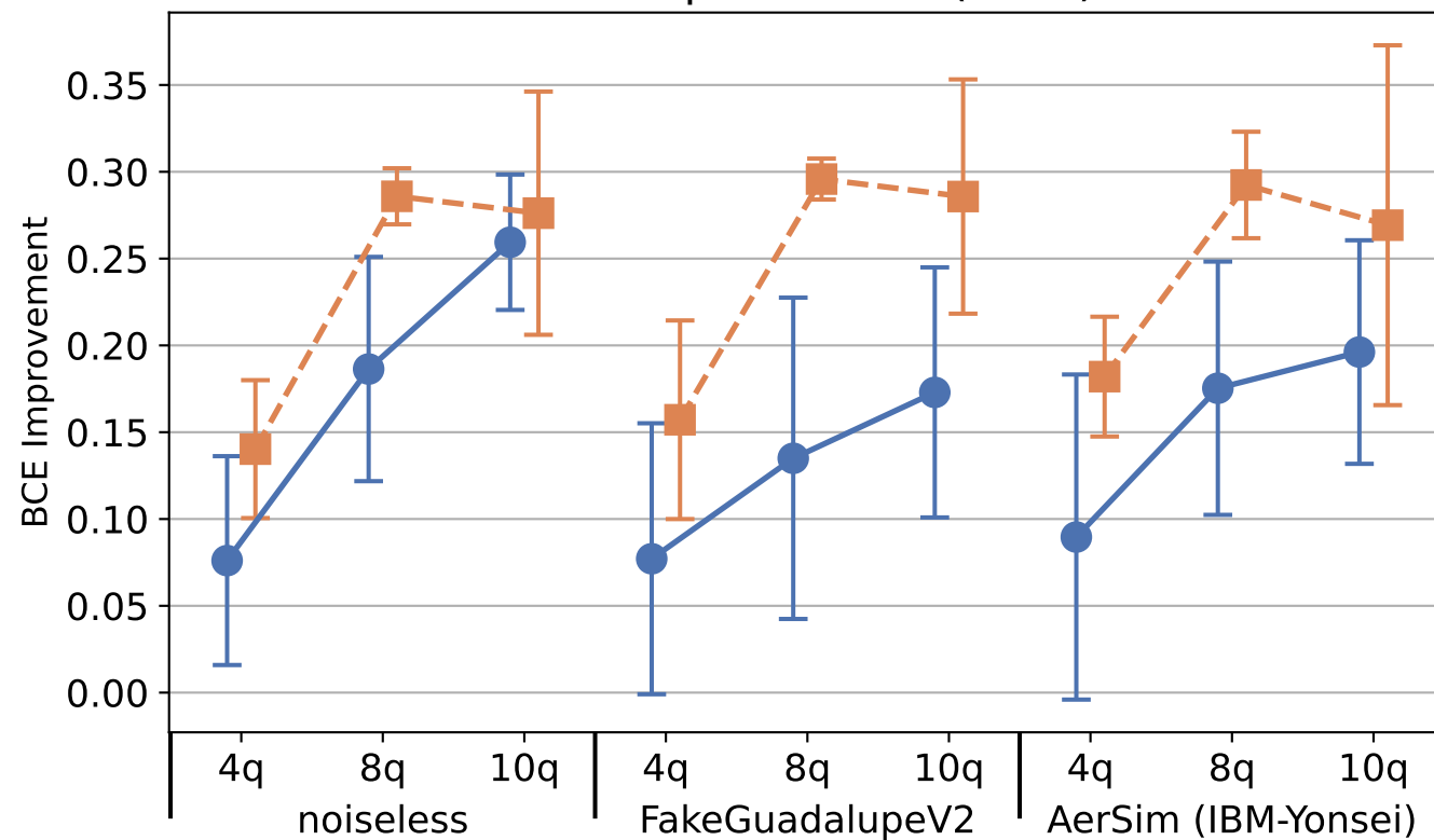
BCE Improvement (Train)
