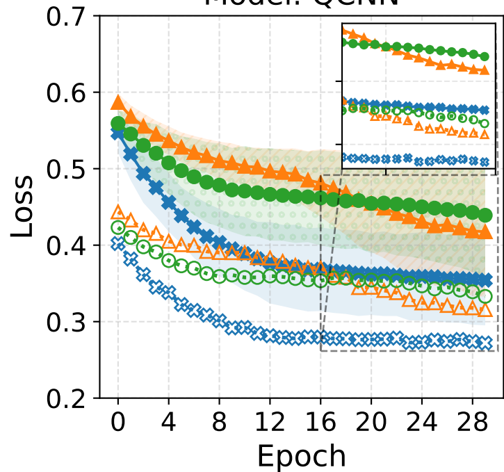
Model: QCNN
