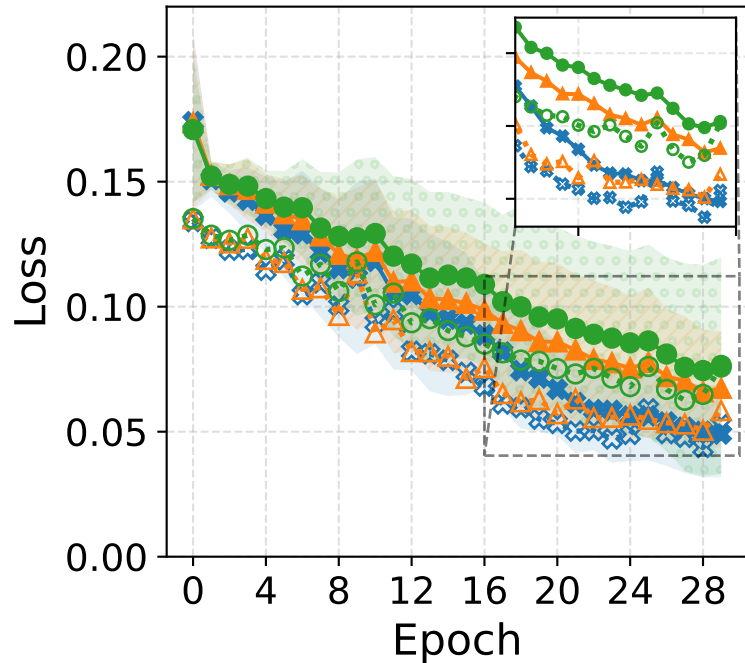
Model: HQCNN-EM
