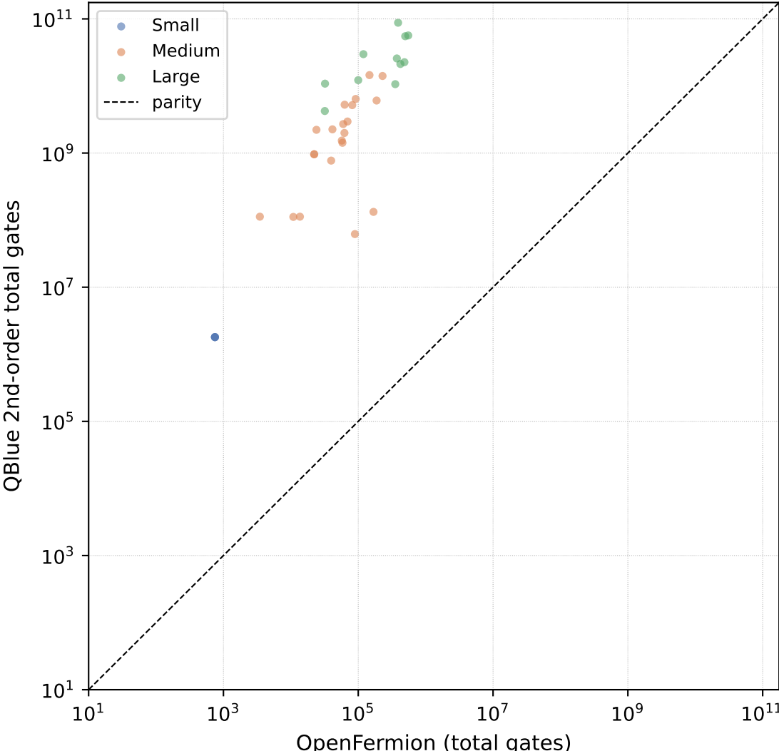
QBlue 2nd-order vs. OpenFermion ( \epsilon=0.1 , t = 0.7854 )
