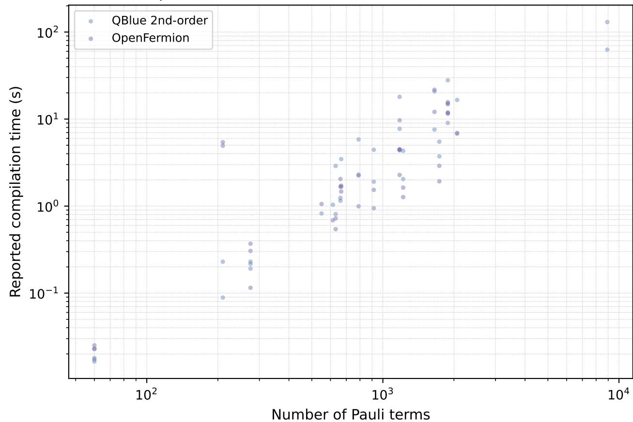
Compilation time vs. Hamiltonian size ( \epsilon=0.1 , t = 0.7854 )
