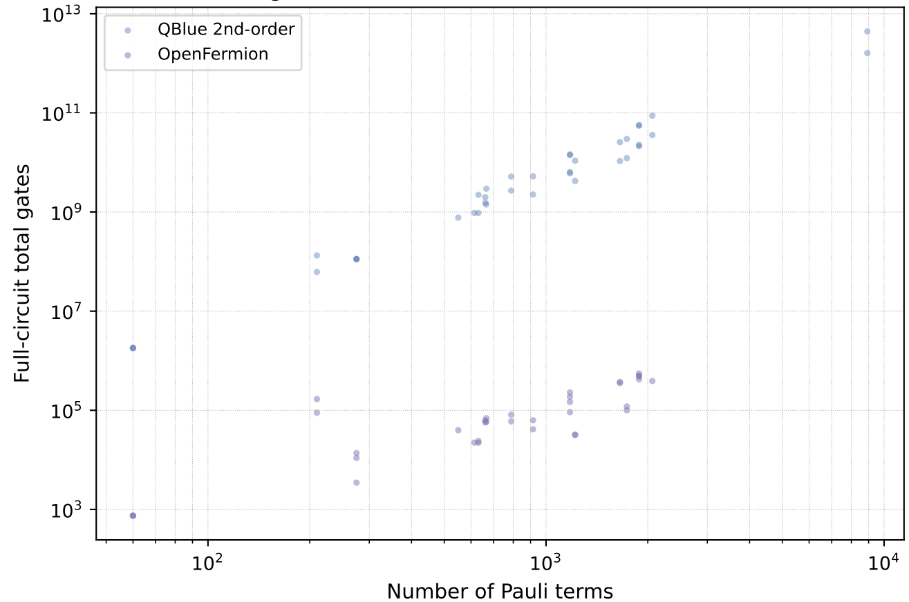
Total gates vs. Hamiltonian size ( \epsilon=0.1 , t = 0.7854 )
