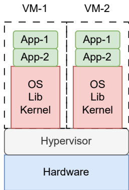
Virtual Machine
