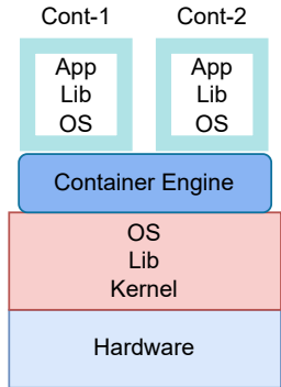
Container
