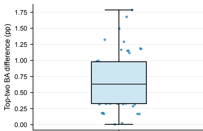
SIPaKMeD / B
