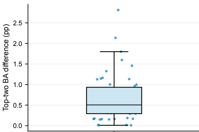
SIPaKMeD / A
