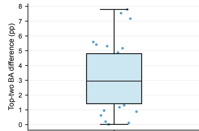
ISIC2019 / A
