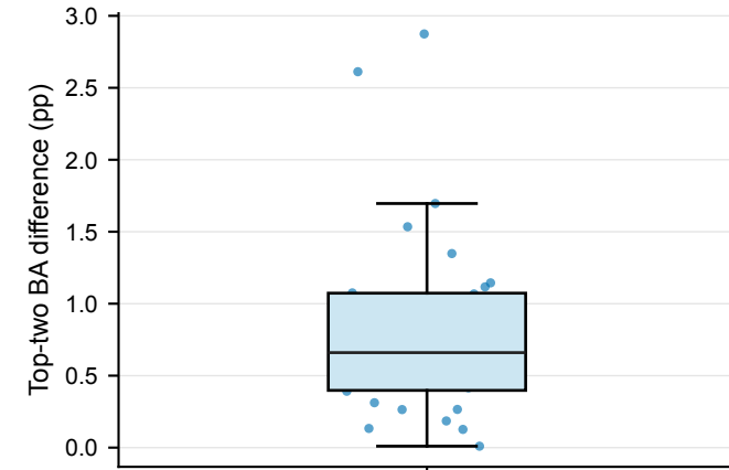
MURA / A
