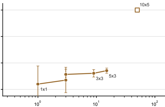
SIPaKMeD / B
