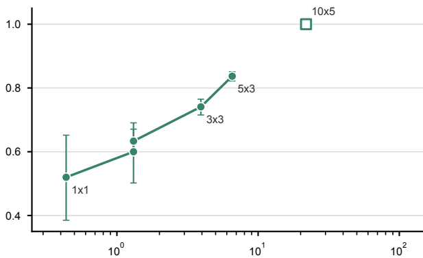
SIPaKMeD / A
