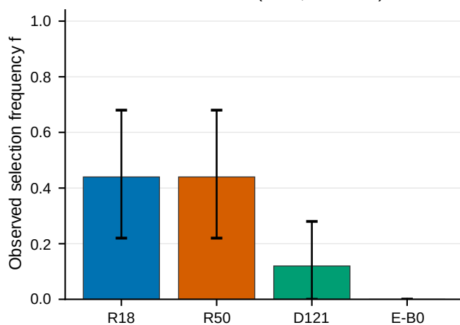
MURA / A (10×3; 4 models)
