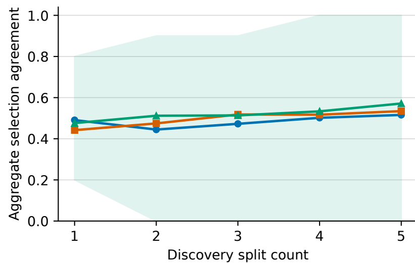
MURA / A (1-3 seeds)
