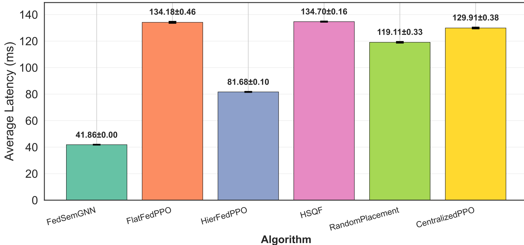
Latency Comparison Across Algorithms [SYSTEM-WISE ANALYSIS: Mean Response Time \pm SE, n=1000 steps]
