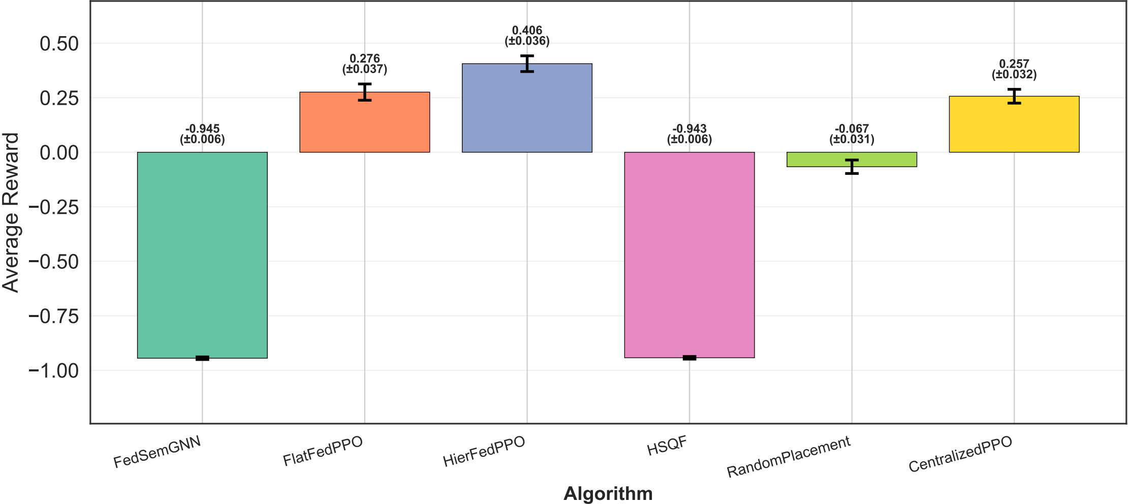
Aggregate Reward Performance Comparison [SYSTEM-WISE ANALYSIS: Mean Performance \pm SE, n=1000 steps]
