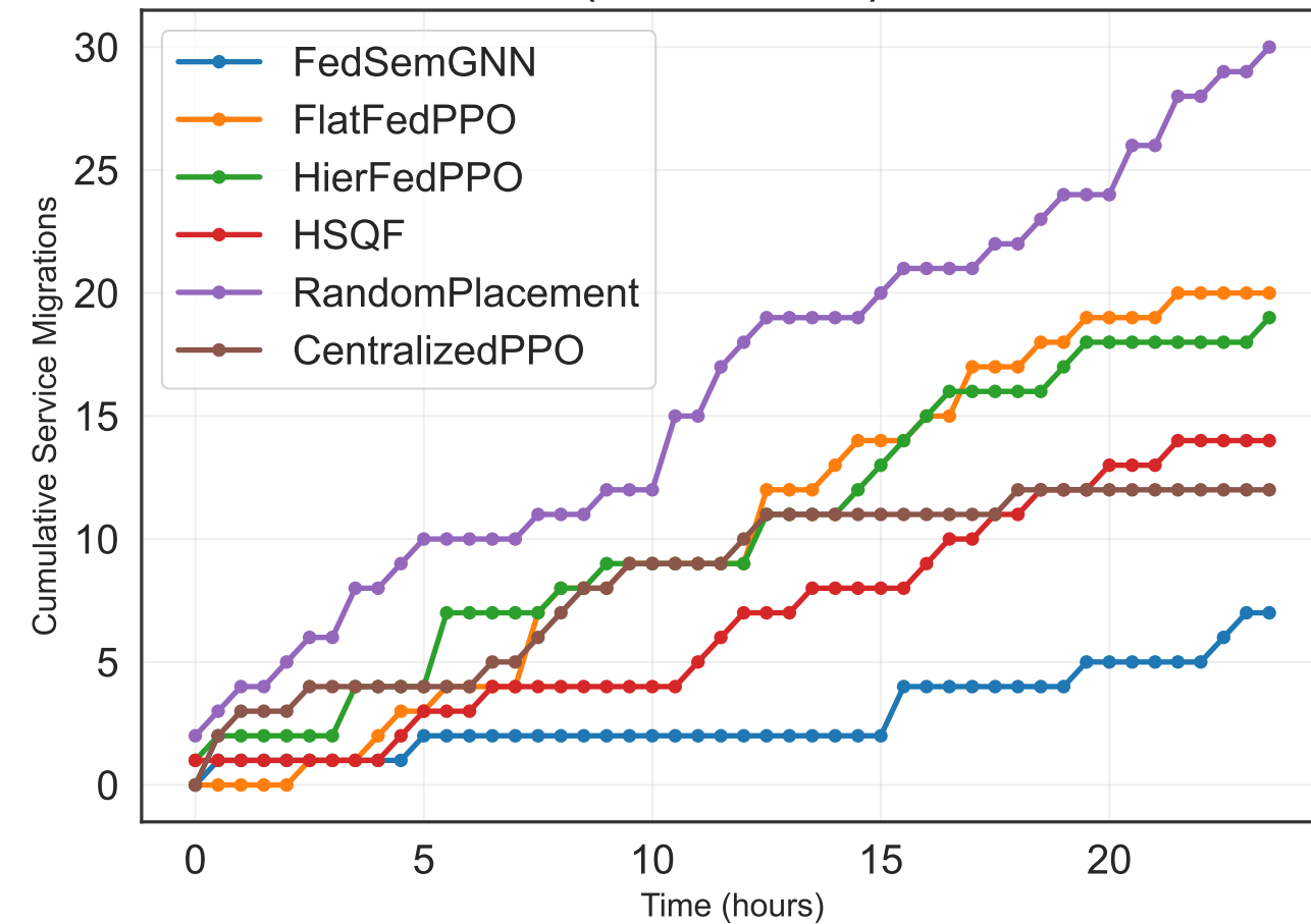
Cumulative Migrations Due to Mobility (24-Hour Period)
