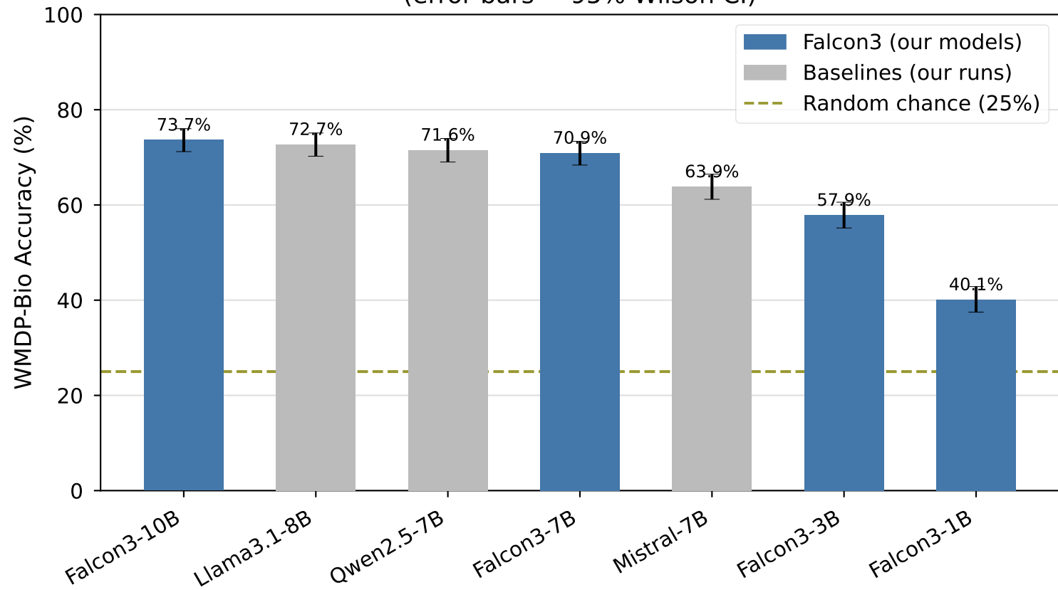
WMDP-Bio Accuracy — Falcon3 Family vs. Baselines (error bars = 95% Wilson CI)
