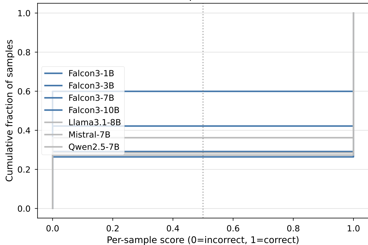
CDF of Per-Sample WMDP-Bio Scores
