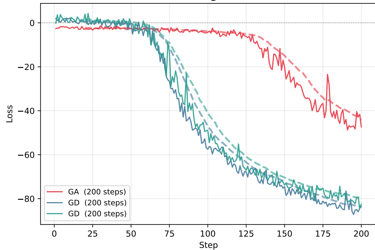
Training Loss
