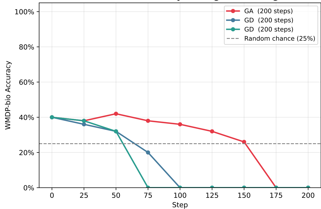
WMDP-bio Accuracy During Unlearning
