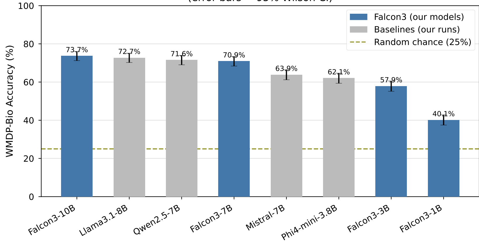
WMDP-Bio Accuracy — Falcon3 Family vs. Baselines (error bars = 95% Wilson CI)
