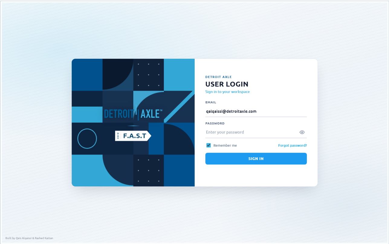
Figure — Login
