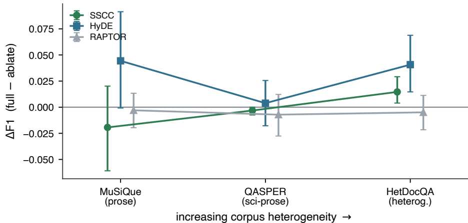
Component benefit vs. corpus heterogeneity
