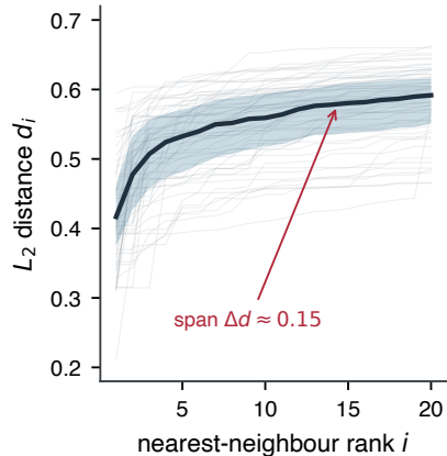
(a) Neighbour distances are near-flat
