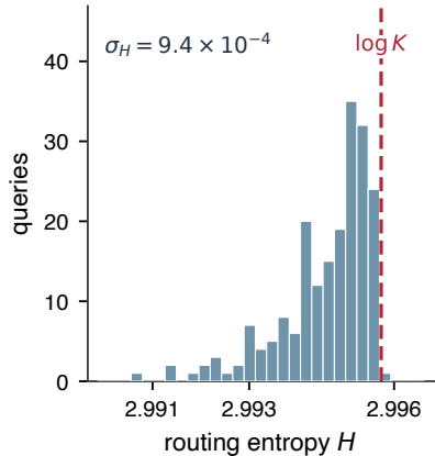
(b) Routing entropy is near-constant
