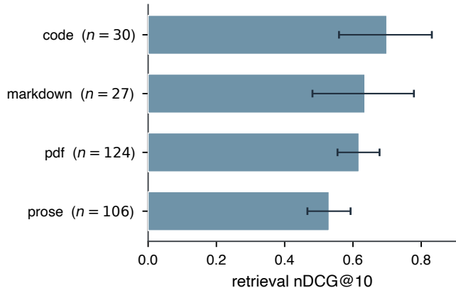
(b) Retrieval by gold-evidence modality
