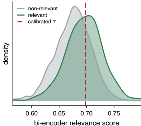
(a) Bi-encoder 1/(1+L_2)
