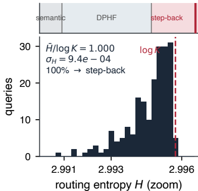
(b) Entropy pinned to the \log K ceiling
