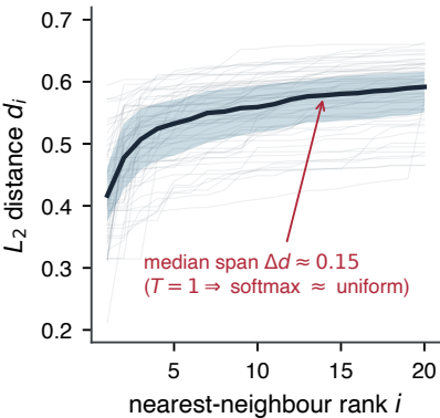
(a) Neighbour distances are near-flat
