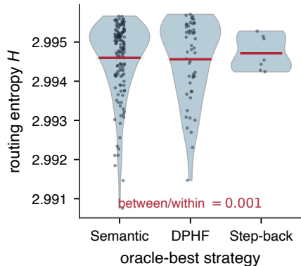
(c) Identical across oracle classes
