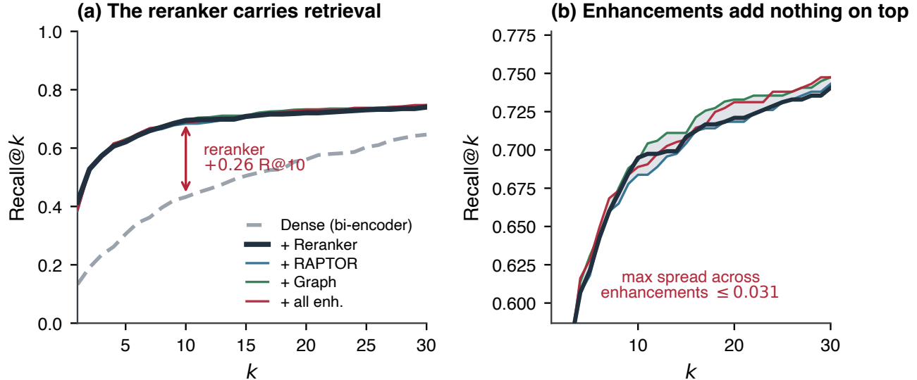
Figure 3: Effect of the reranker on recall. Recall@ k on HetDocQA dev, with all configurations sharing the same first-stage retriever. Adding the cross-encoder reranker raises the curve sharply, whereas adding the pool-expansion methods (RAPTOR, graph, and all combined) on top of the reranker changes it little.
