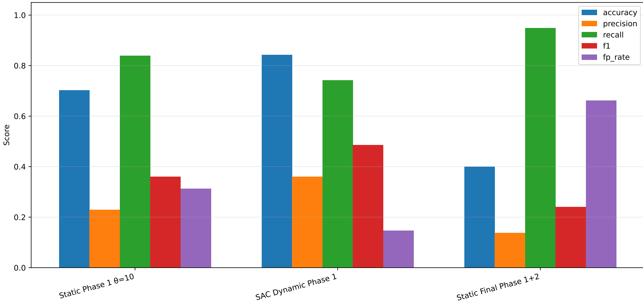
Random 10% Attack: Static vs SAC Dynamic Threshold Comparison
