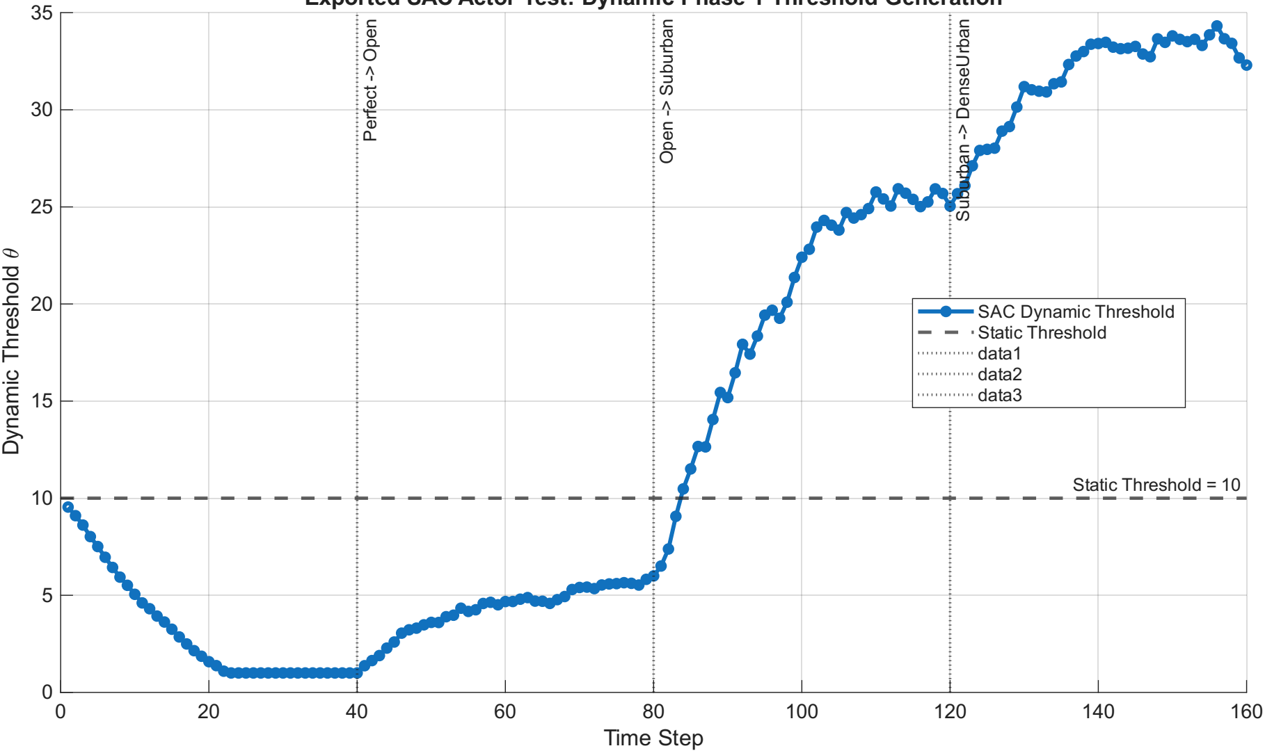
Exported SAC Actor Test: Dynamic Phase 1 Threshold Generation
