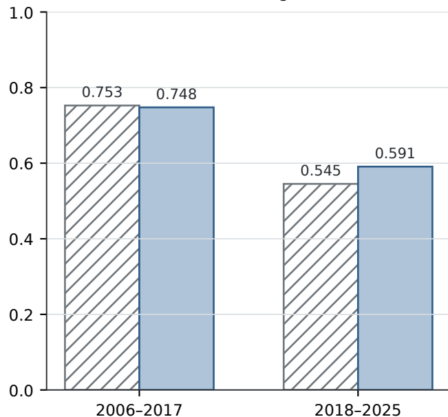
Panel B. ROC-AUC (higher is better)
