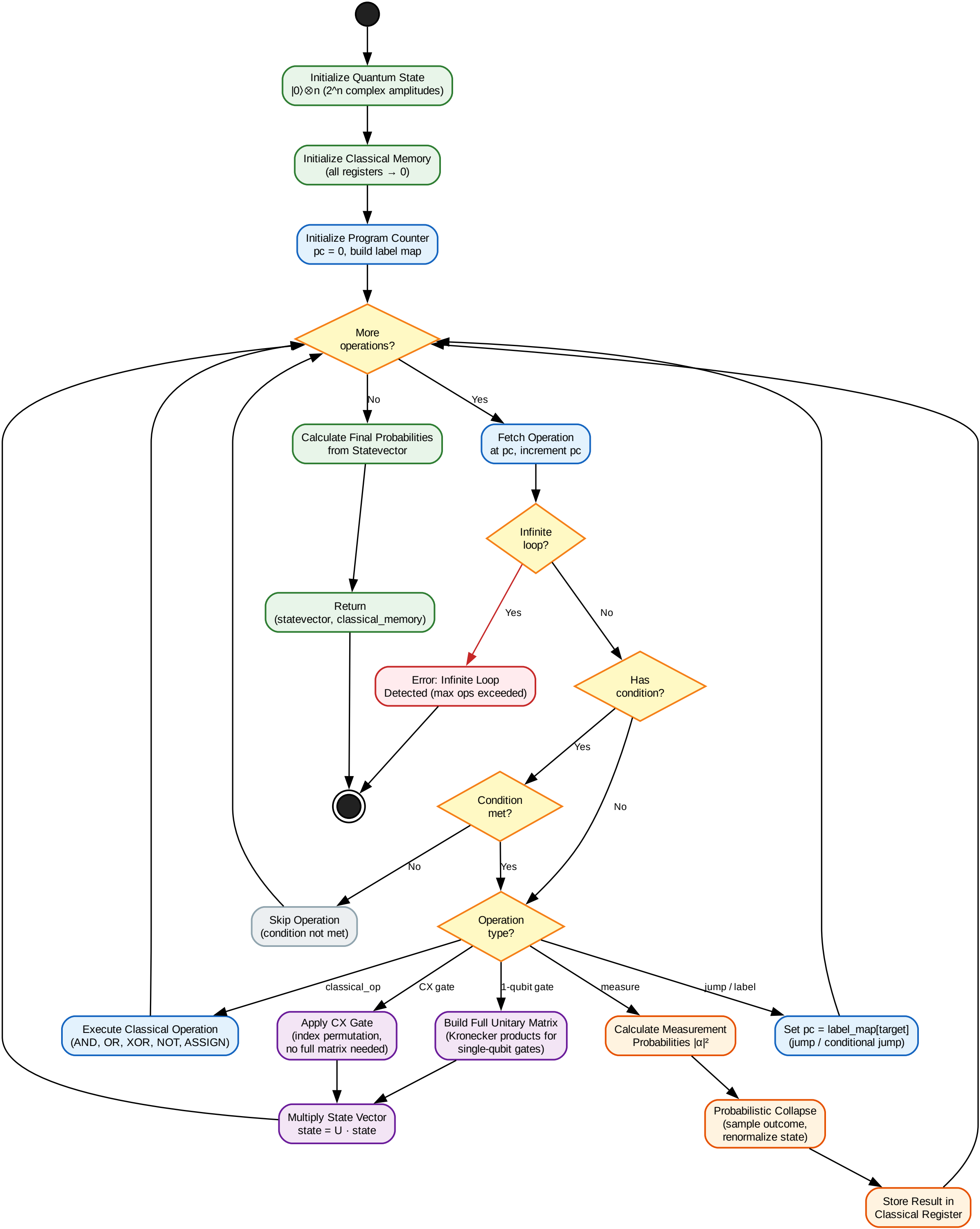
Activity Diagram — Simulation Process
