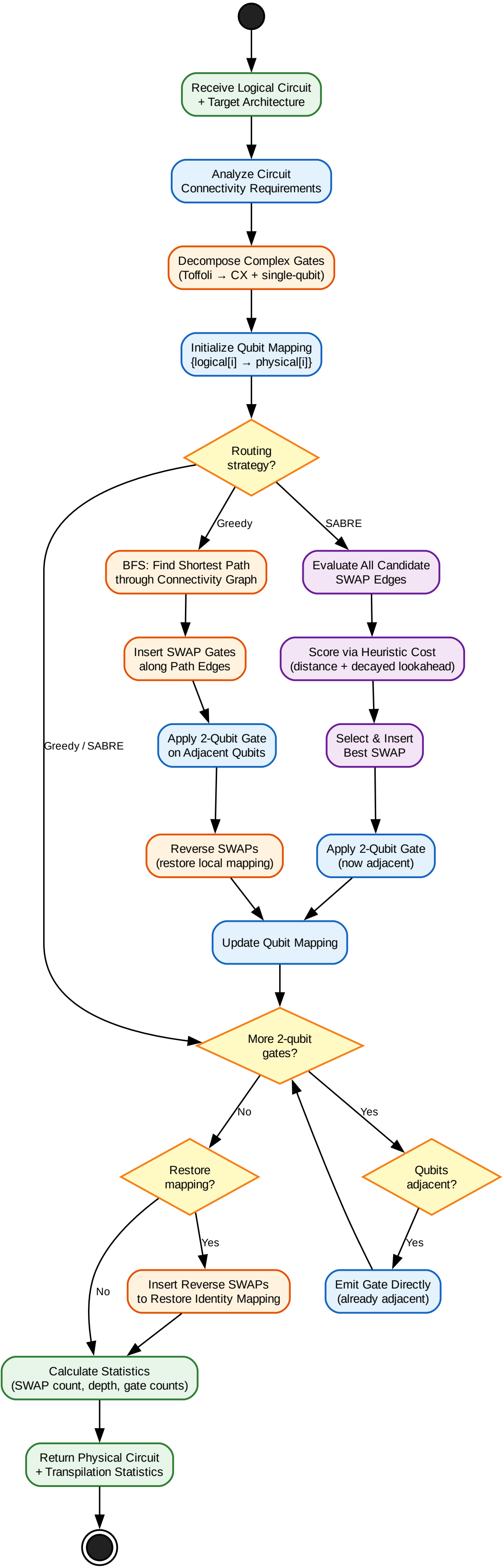
Activity Diagram — Transpilation Process
