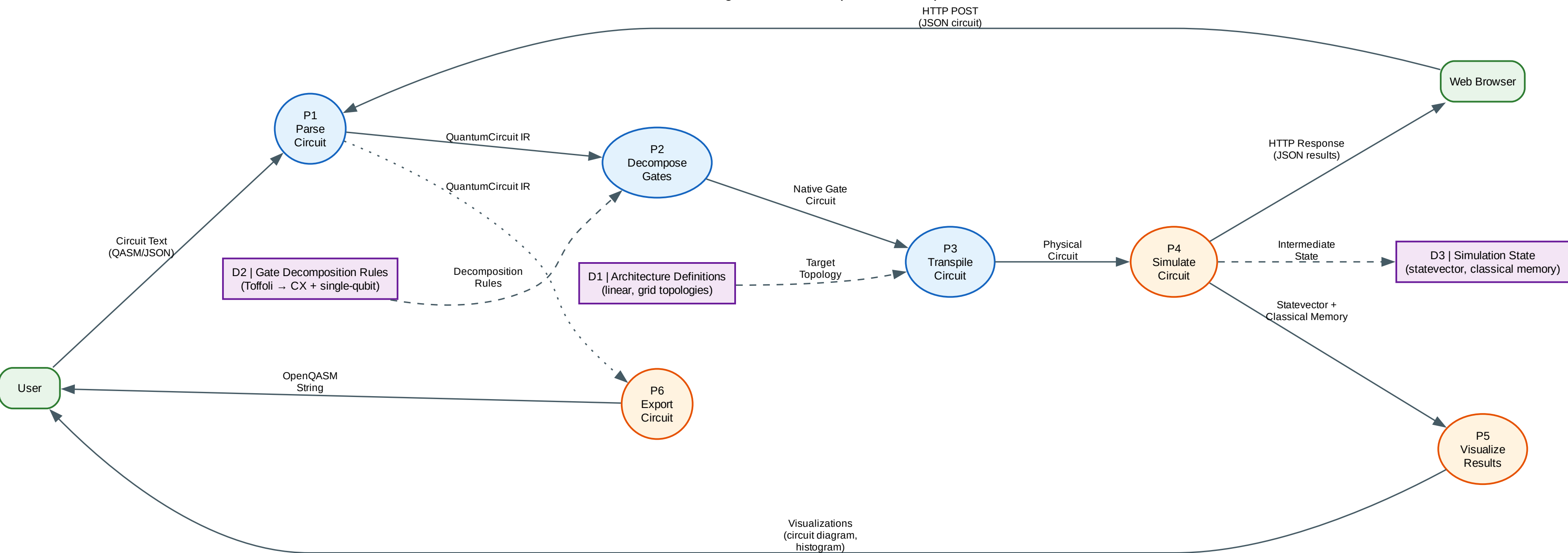
Data Flow Diagram — Level 2 (Module Level)
