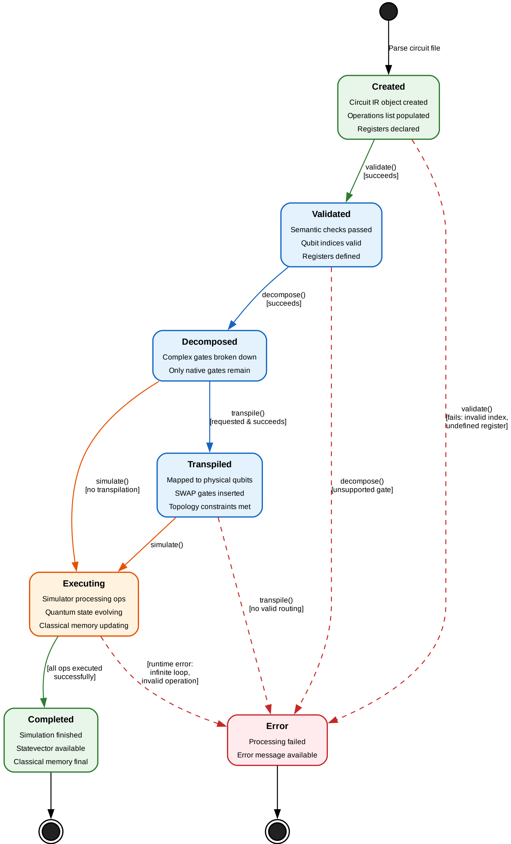
Circuit Lifecycle State Transition Diagram
