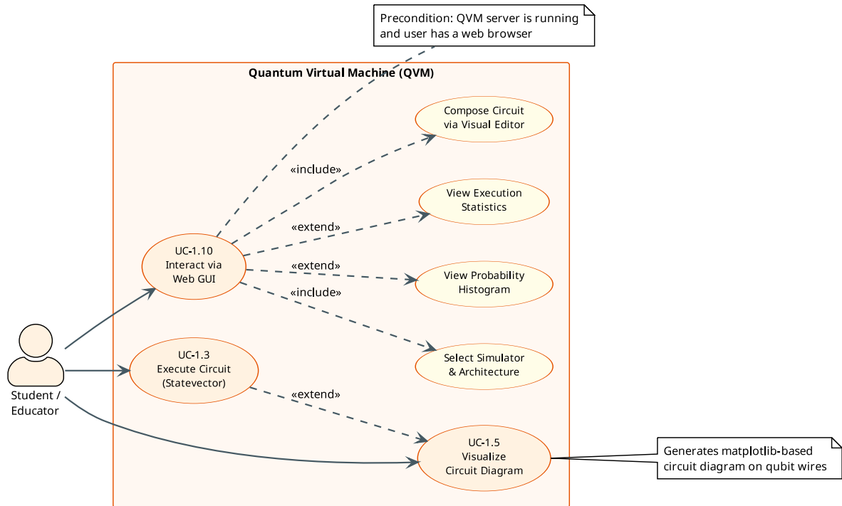
Figure 3.3: Use Case Diagram — Student / Educator
