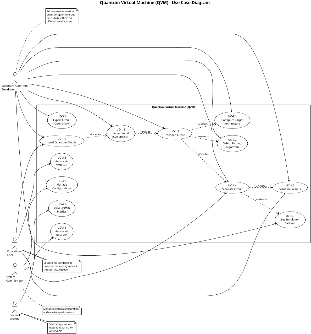
Figure 3.1: Combined Use Case Diagram for Quantum Virtual Machine
