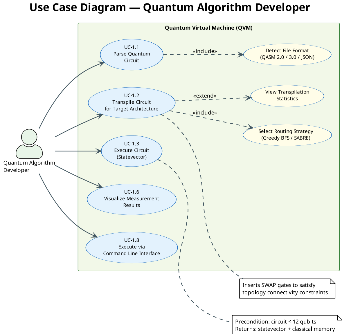
Figure 3.2: Use Case Diagram — Quantum Algorithm Developer
