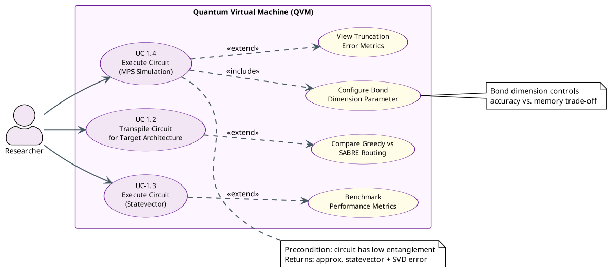
Figure 3.4: Use Case Diagram — Researcher
