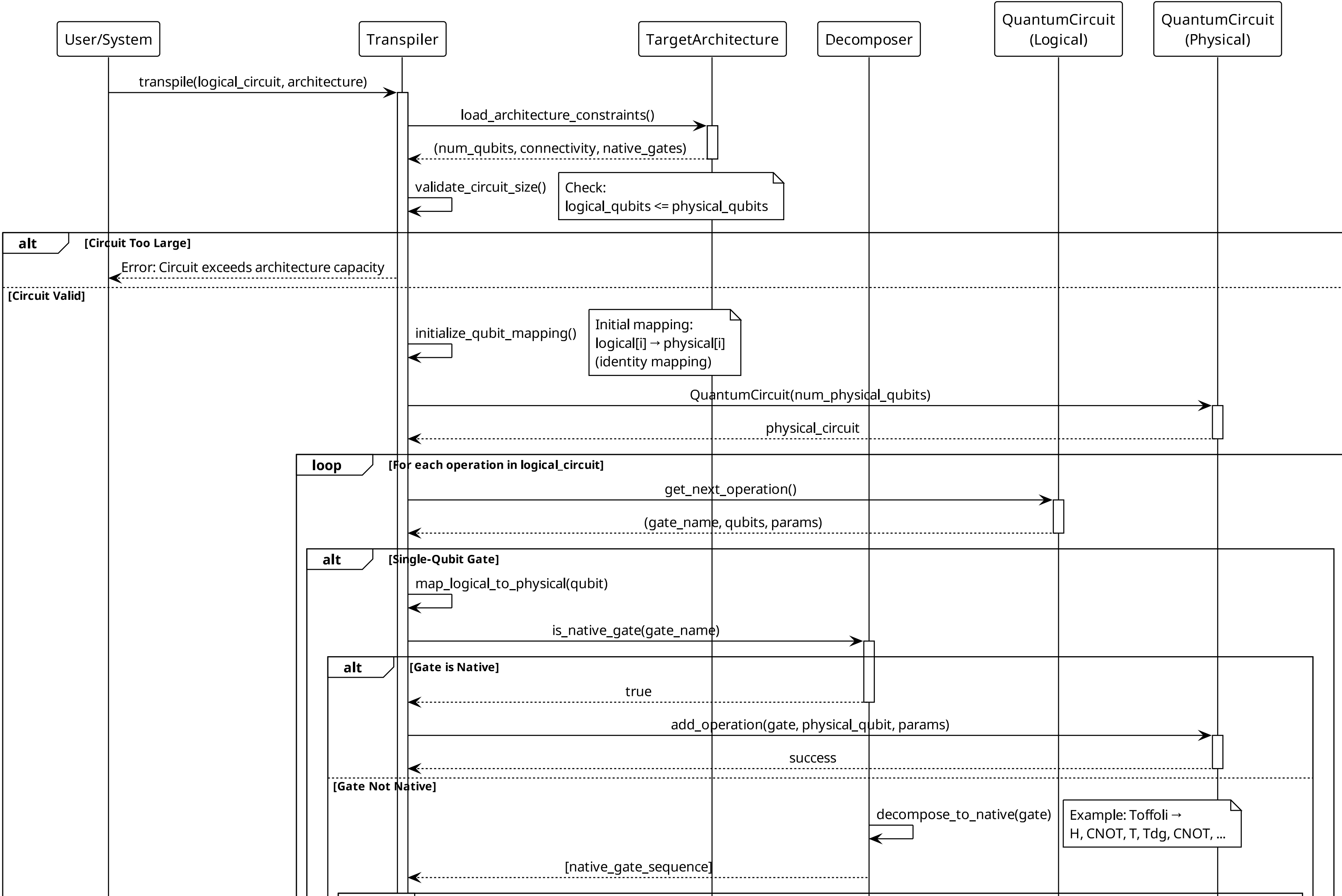
Sequence Diagram - Transpilation Process (Detailed)
