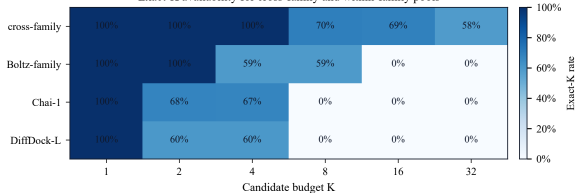
Exact-K availability for cross-family and within-family pools
