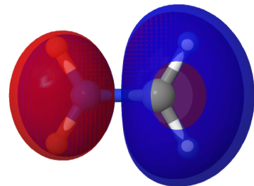
MO 9 (virt.) -0.146 E_h
