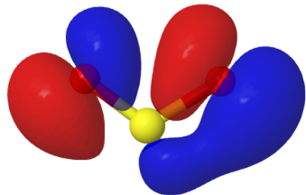
MO 14 (occ.) -0.511 E_h
