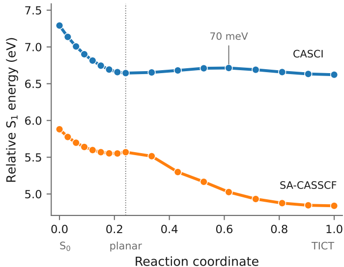
(a) CASCI geometries
