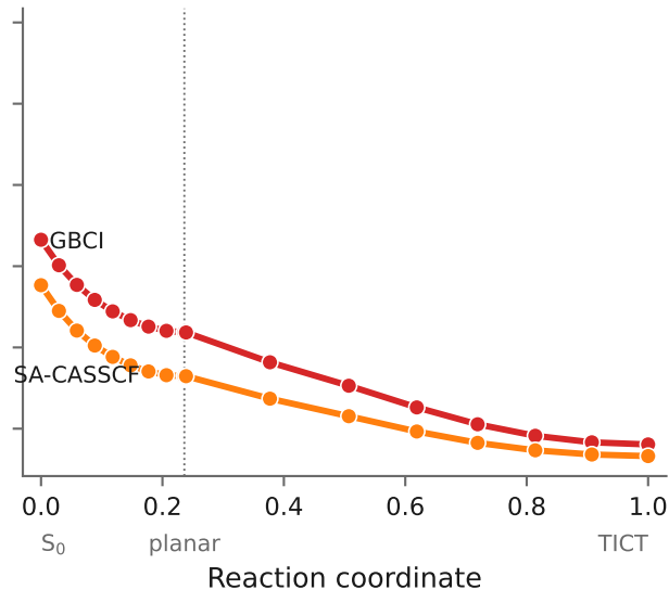
(b) GBCI geometries
