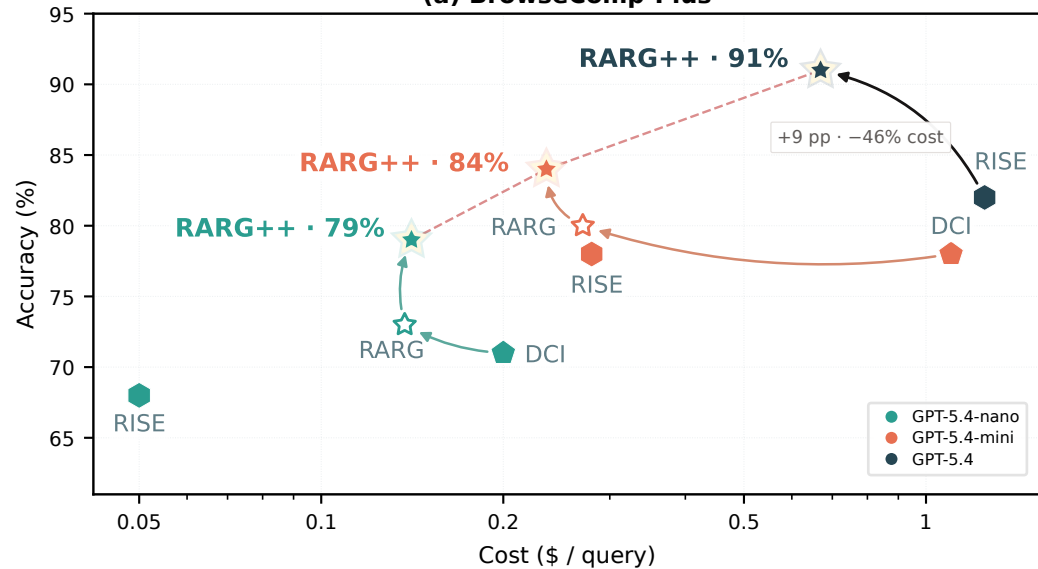
(a) BrowseComp-Plus
