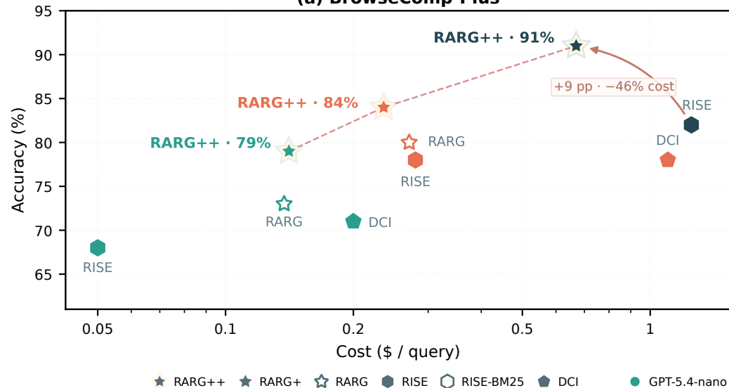
(a) BrowseComp-Plus
