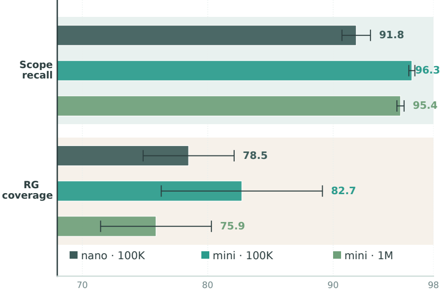
(a) Scope Recall and RG Coverage
