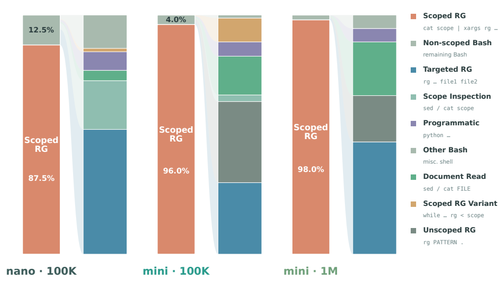
(b) Bash Command Composition
